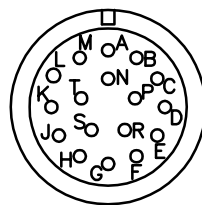
17 pole plug (MS3102A20-29P) (Multi Turn Encoder Connector Pins)
