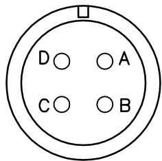
(사양:MS3102A32-17P) (Power Connector Pin Map)
