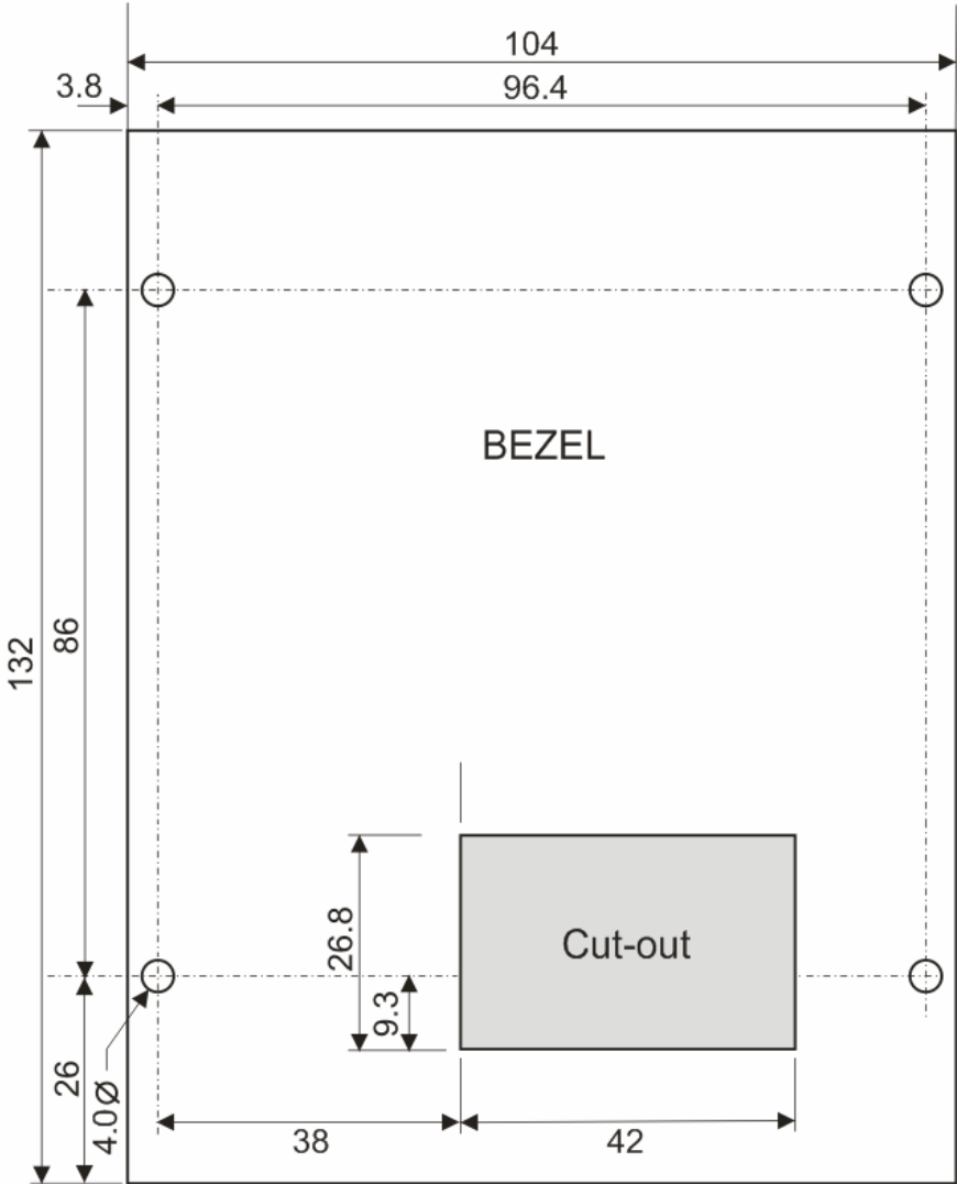
Mounting Dimensions for the Remote-Mounted 6911 Keypad
